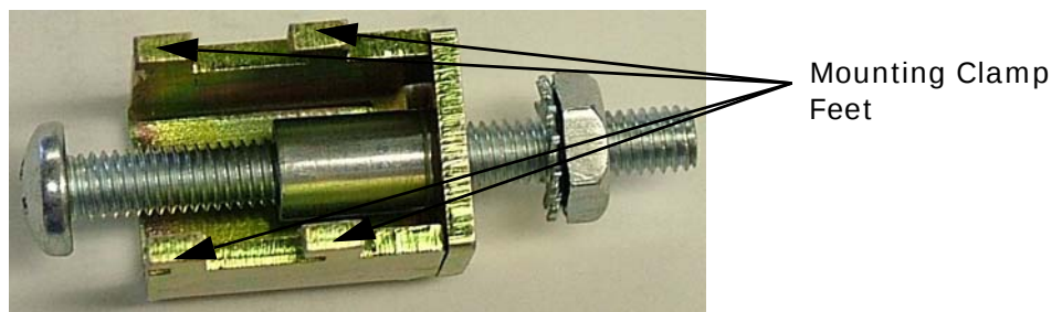
Figure 2-4: Mounting Clamp
