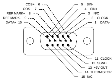
Absolute Encoder
